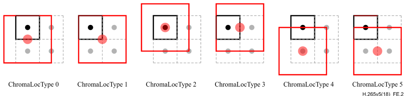
Figure E.2 – Location of the top-left chroma sample when chroma_format_idc is equal to 1 (4:2:0 chroma format) as a function of ChromaLocType
